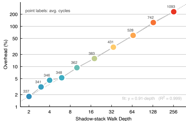
Figure 3. Per-frame shadow-stack walk cost. Overhead scales linearly with walk depth ( \approx 0.91\% per frame, R^2 = 0.999 ). Marker color encodes overhead magnitude; numbers above each point are the raw cycle counts.
