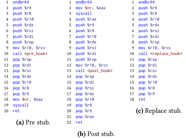
Figure 2. Trampoline stub variants.
